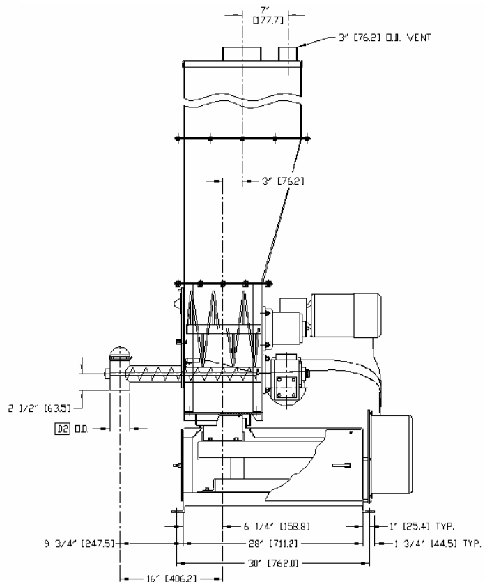
HOPPER EXTENSION
